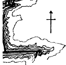
Map of the gorge of the river below the Victoria Falls (Lampugh).
